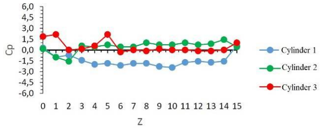
(b) Model II serial configuration, M/D and N/D=0.6 on Re=43,844
