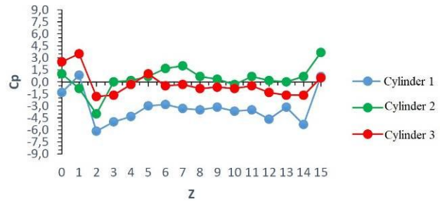
(c) Model II parallel configuration, M/D and N/D=1.2 at Re=43,844
