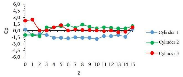
(a) Model II serial configuration, M/D and N/D=0.0 on Re=43,844
