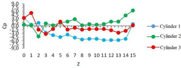
(a) Model I parallel configuration, M/D=0.0 at Re=43,844
