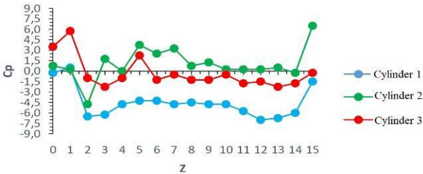
(b) Model I parallel configuration, M/D=0.6 at Re=43,844
