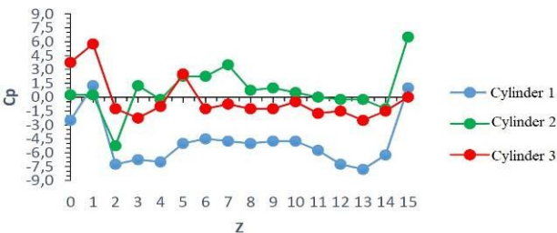
(c) Model I parallel configuration, M/D=1,2 at Re=43,844
