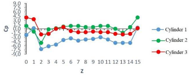
(b) Model II parallel configuration, M/D and N/D=0.6 at Re=43,844
