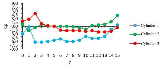
(a) Model II parallel configuration, M/D and N/D=0.0 at Re=43,844
